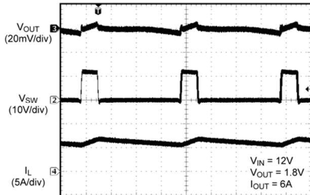
Switching Waveforms; IOUT = 6A
