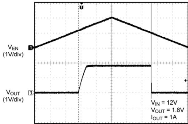
Time (10ms/div)
